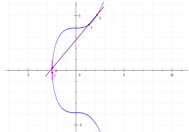
Elliptic Curve ( y^2 \bmod p = (x^2 + ax + b) \bmod p ), Curve Size : Small ,Curve Type : F(p)
