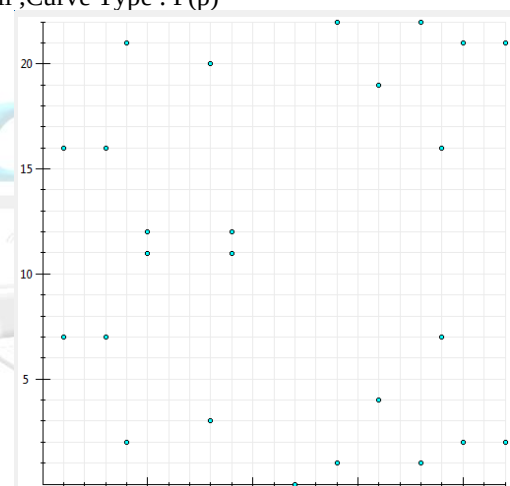
Elliptic Curve ( y^2 \bmod p = (x^2 + ax + b) \bmod p ), Curve Size : Small ,Curve Type : F(p)
