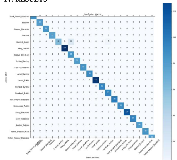
Figure 2. The confusion matrix for the classification model.
